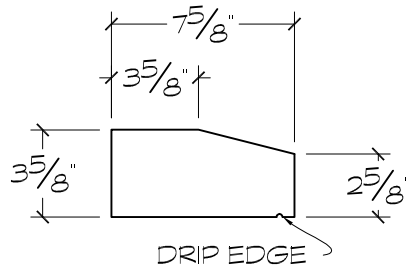
CROSS SECTION
